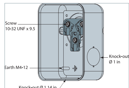
Terminal box for model (2)
