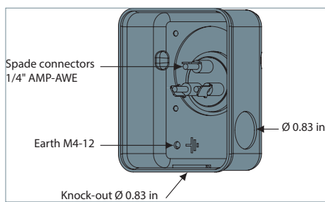
Terminal box for model (1)
