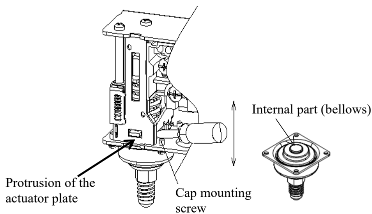
Pressure switch low-pressure side
