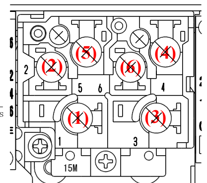
Micro switch terminal numbers and positions (The number of terminals varies depending on the model.)
