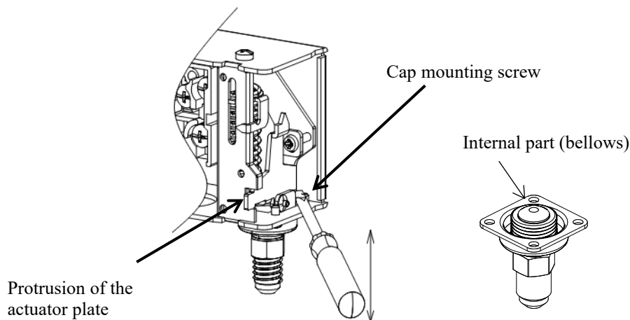
Pressure switch high-pressure side
