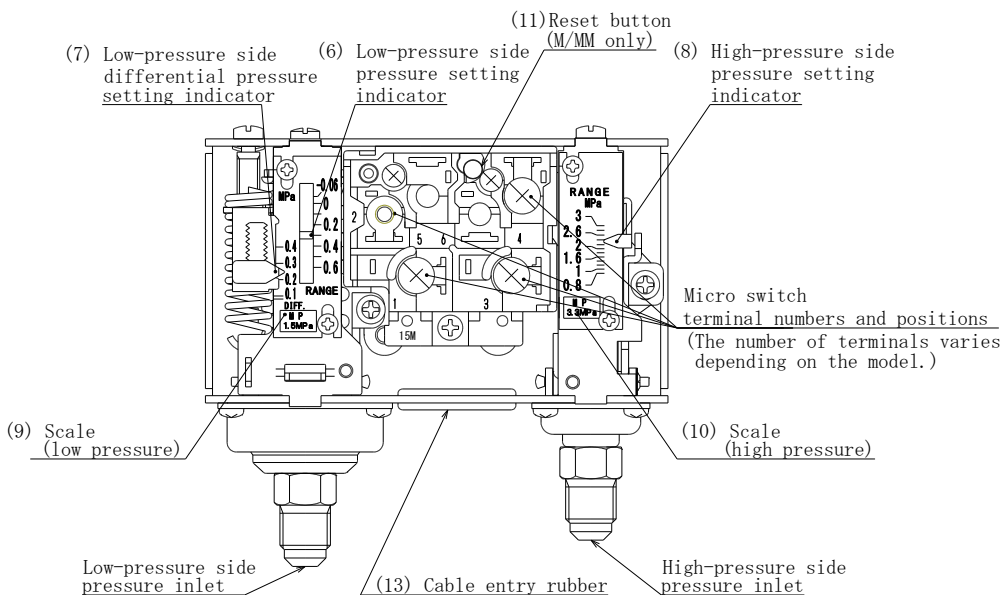
Micro switch terminal numbers and positions (The number of terminals varies depending on the model.)
