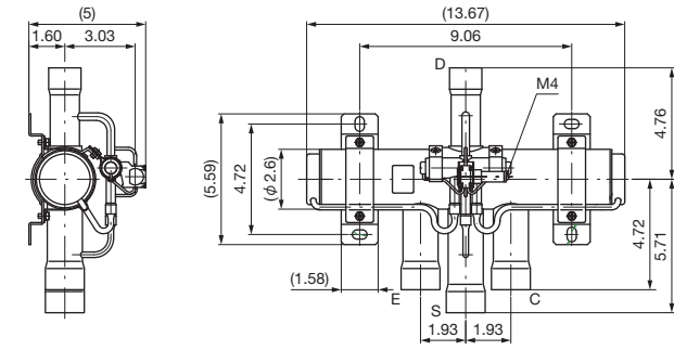
Type STF-30U19G
